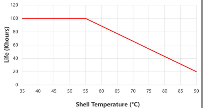
Life - Shell Temperature Curve
